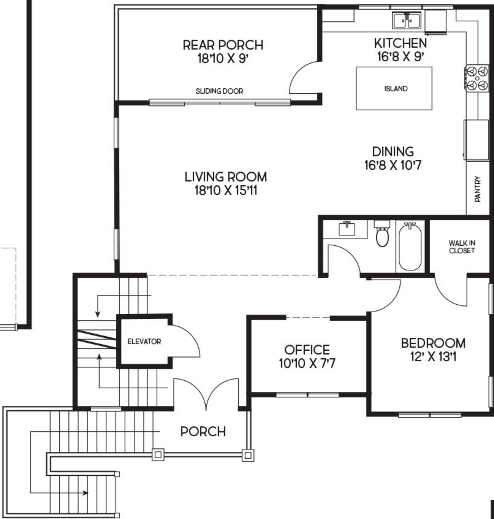
FIRST FLOOR - 1132 HEATED SQ. FT.
