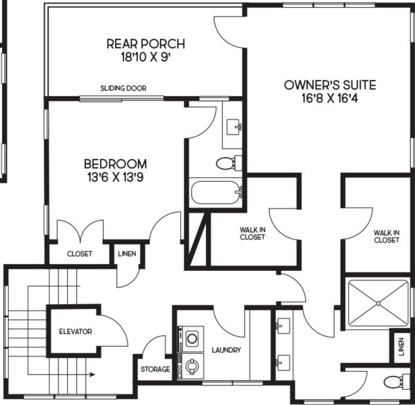
SECOND FLOOR - 1115 HEATED SQ. FT.
